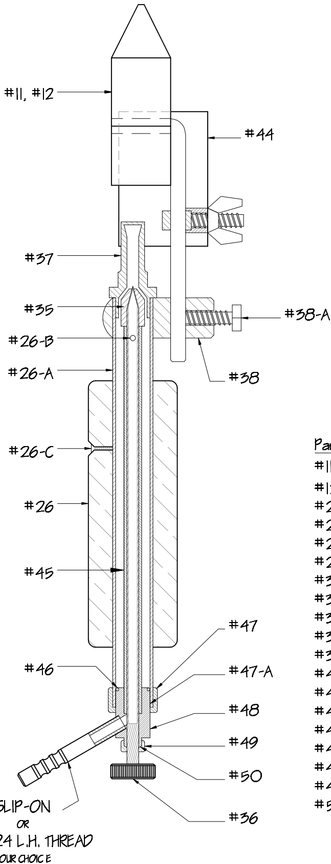
AERO Duplex Soldering Torch
