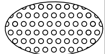
Front View of Perforated Copper 3/32" Perforated w/ 5/32" Staggered Centers
