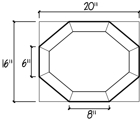
Plan/Top View
