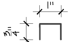
FRONT VIEW OF SUPPORT BRACKET
