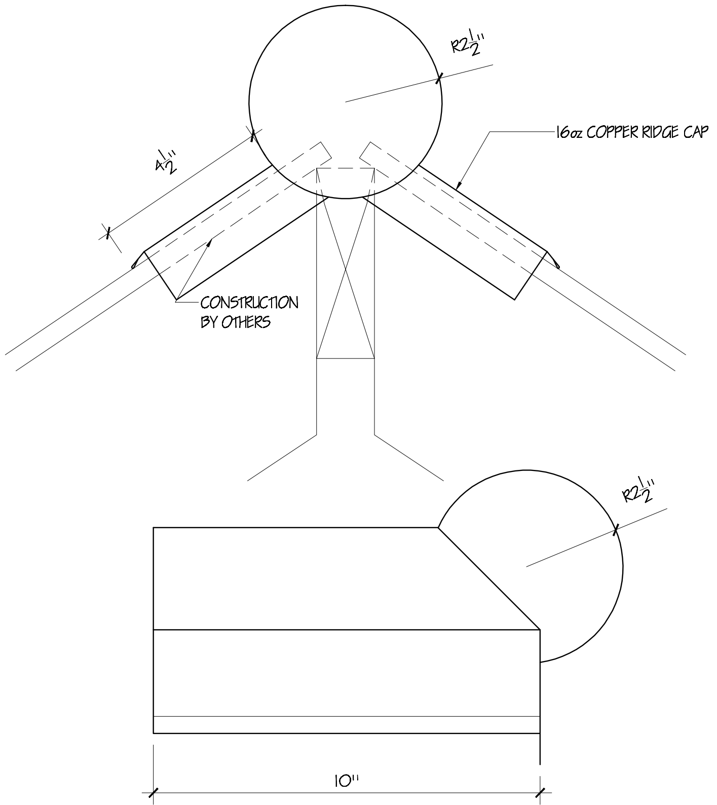
SIDE ELEVATION
