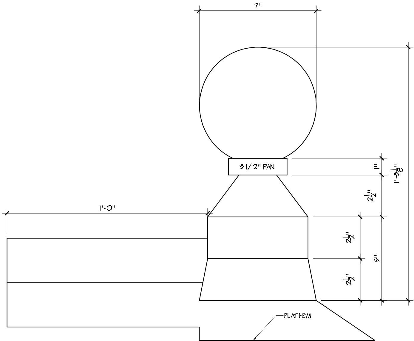
SIDE ELEVATION
