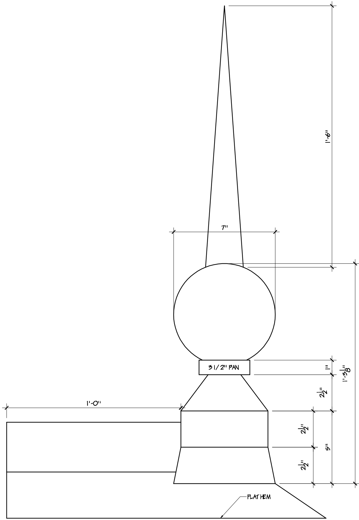
SIDE ELEVATION
