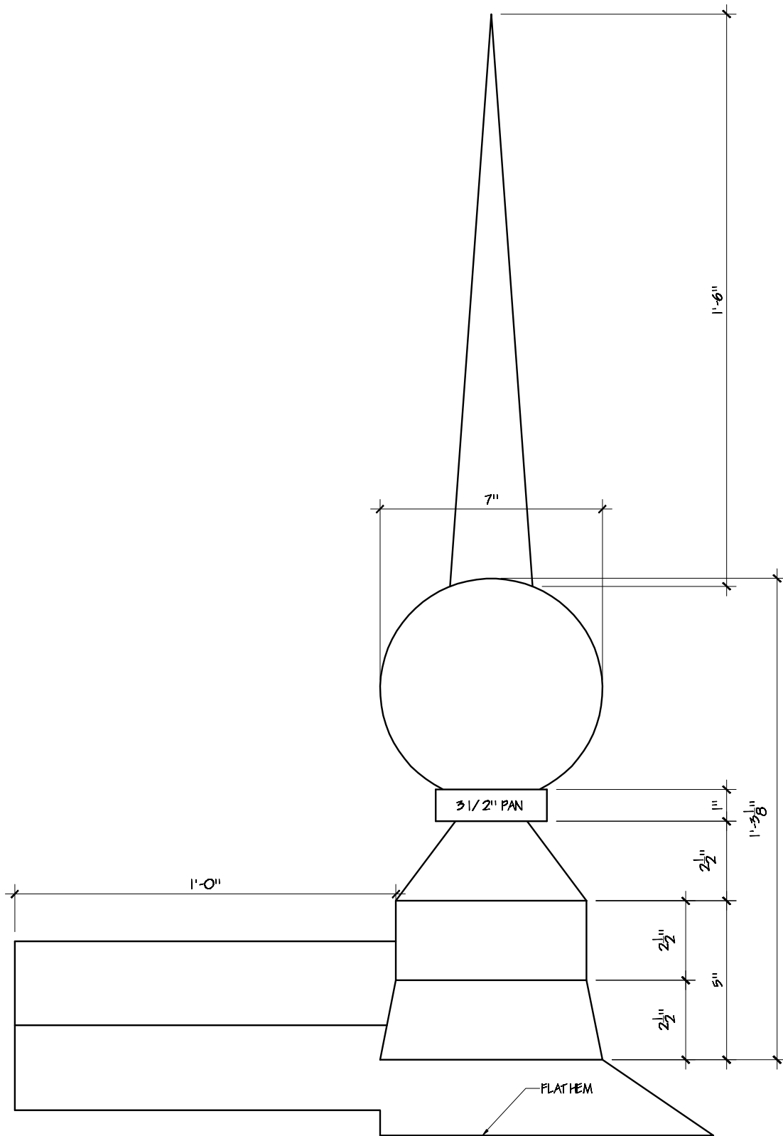
SIDE ELEVATION
