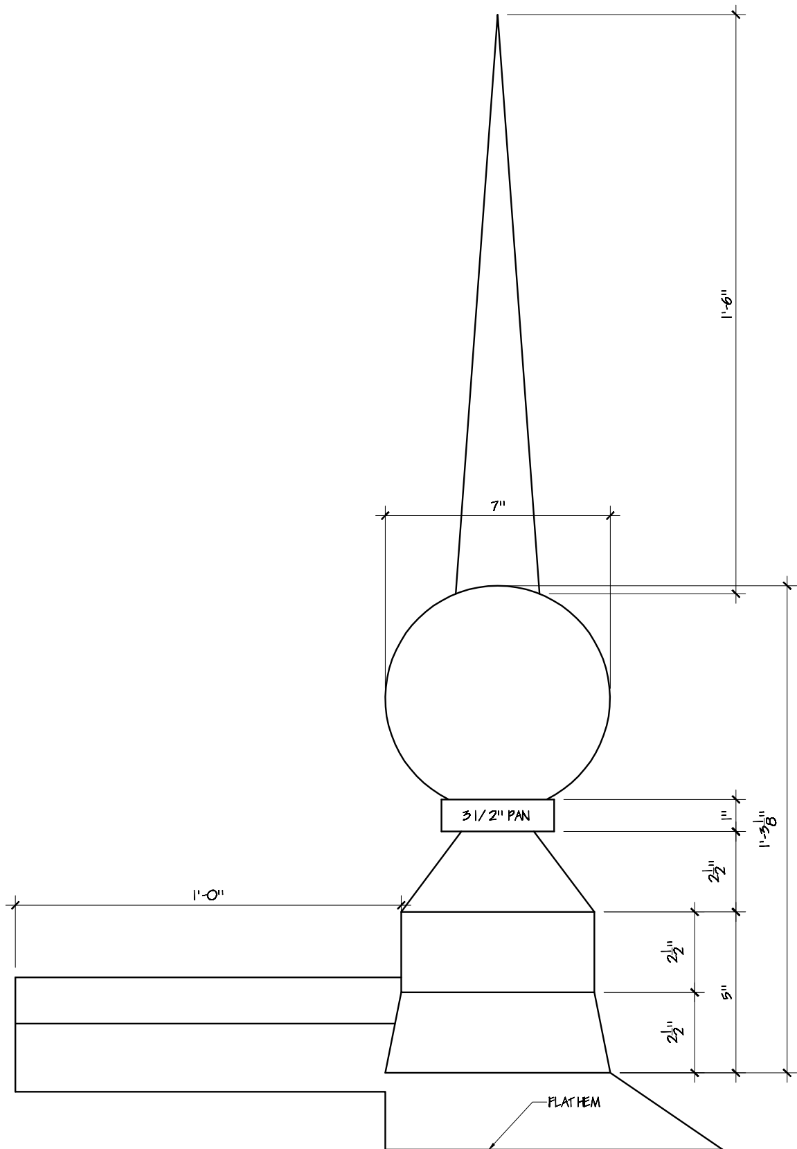
SIDE ELEVATION
