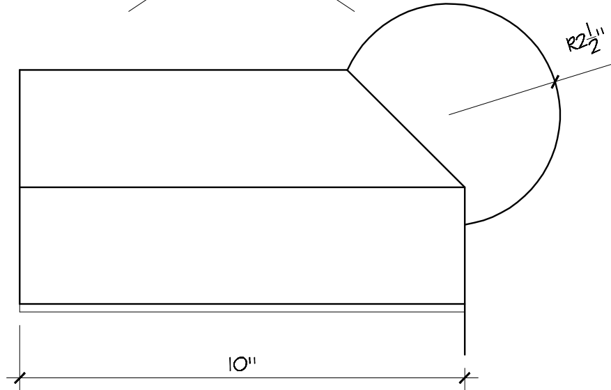
SIDE ELEVATION
