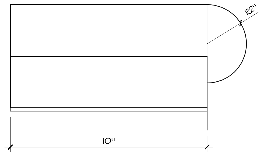
SIDE ELEVATION
