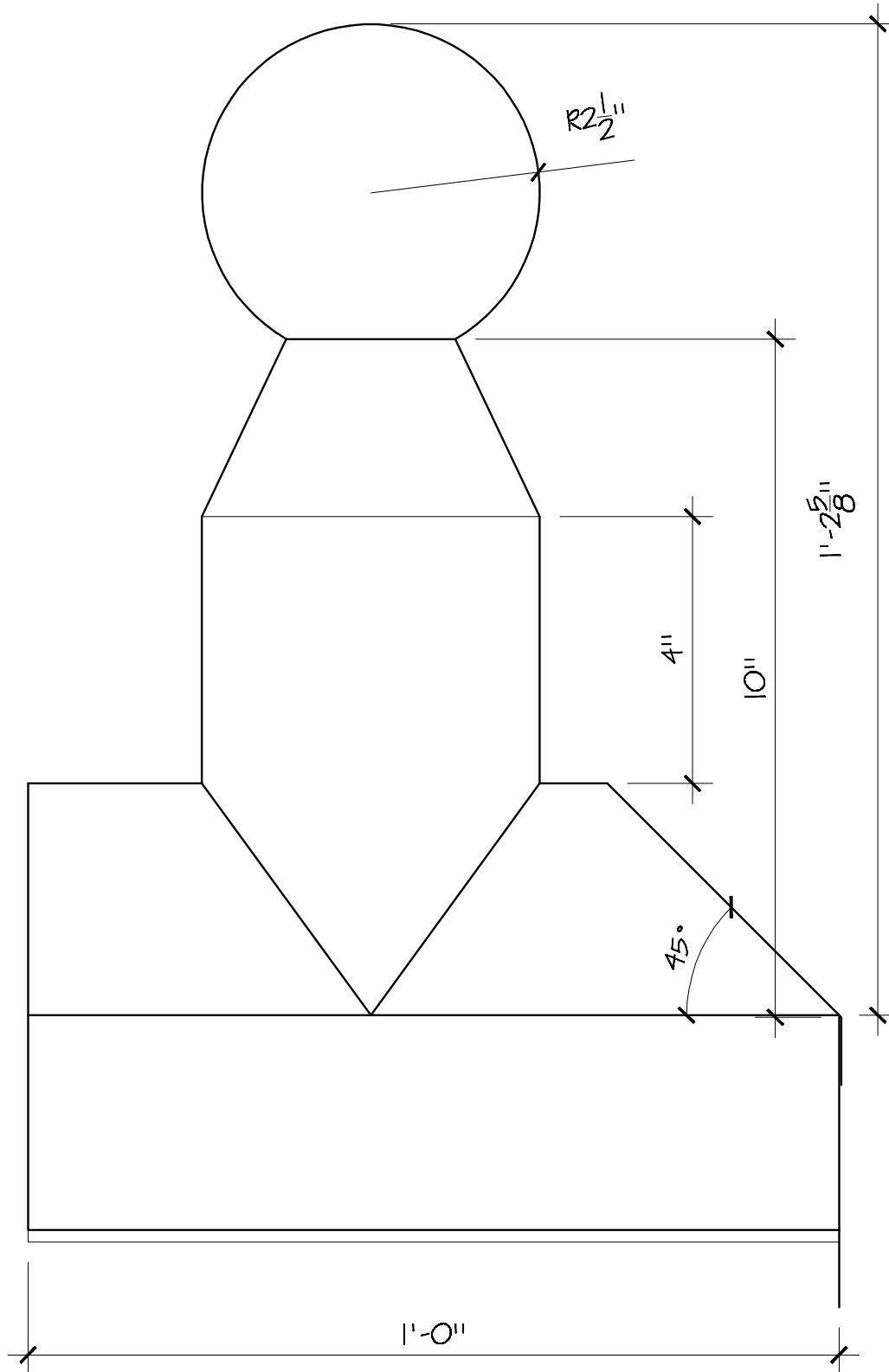
SIDE ELEVATION
