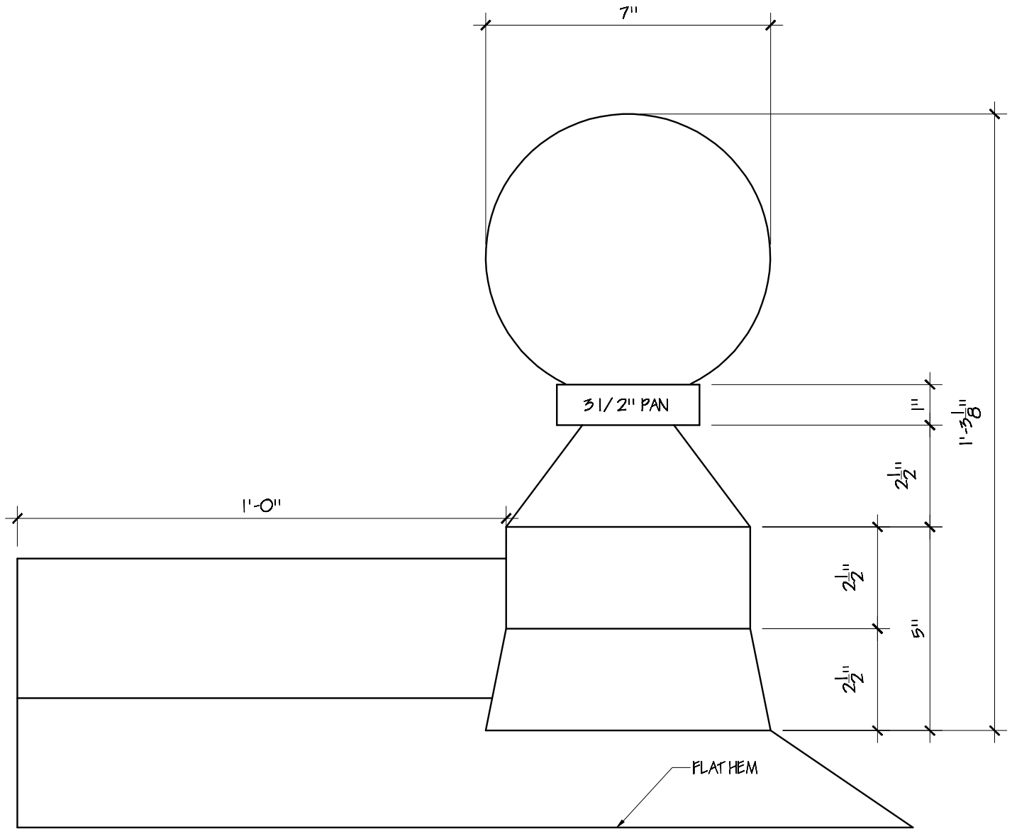
SIDE ELEVATION
