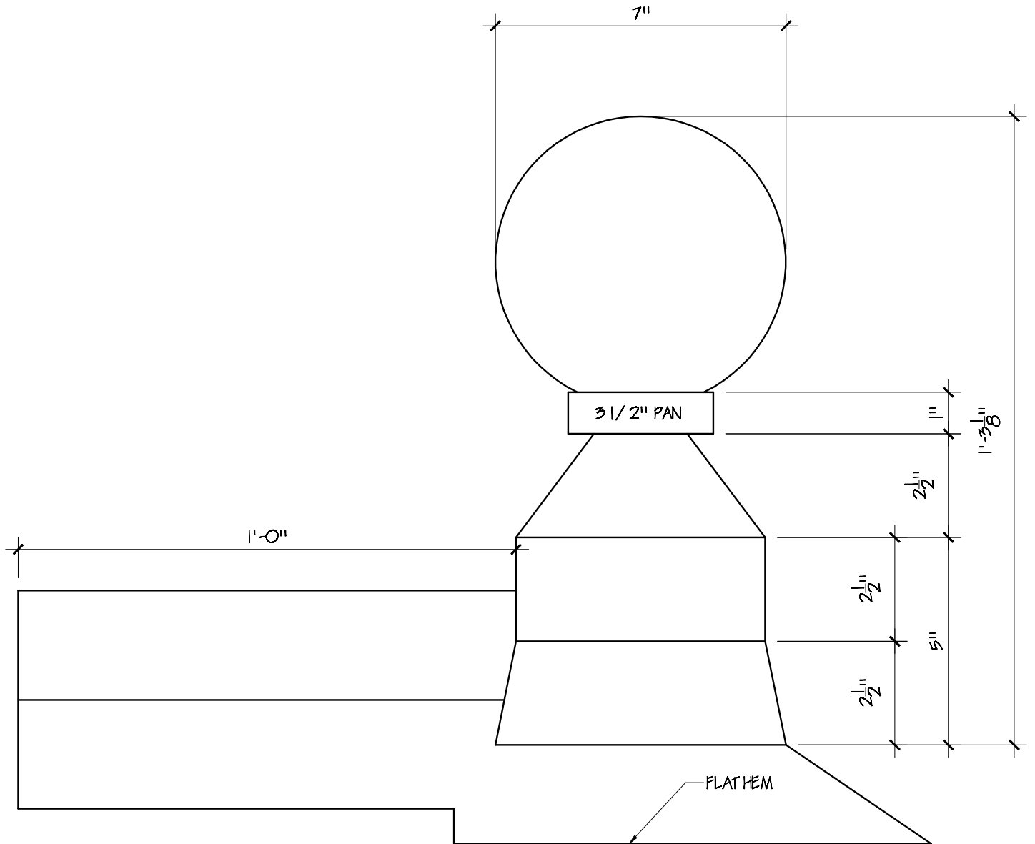
SIDE ELEVATION
