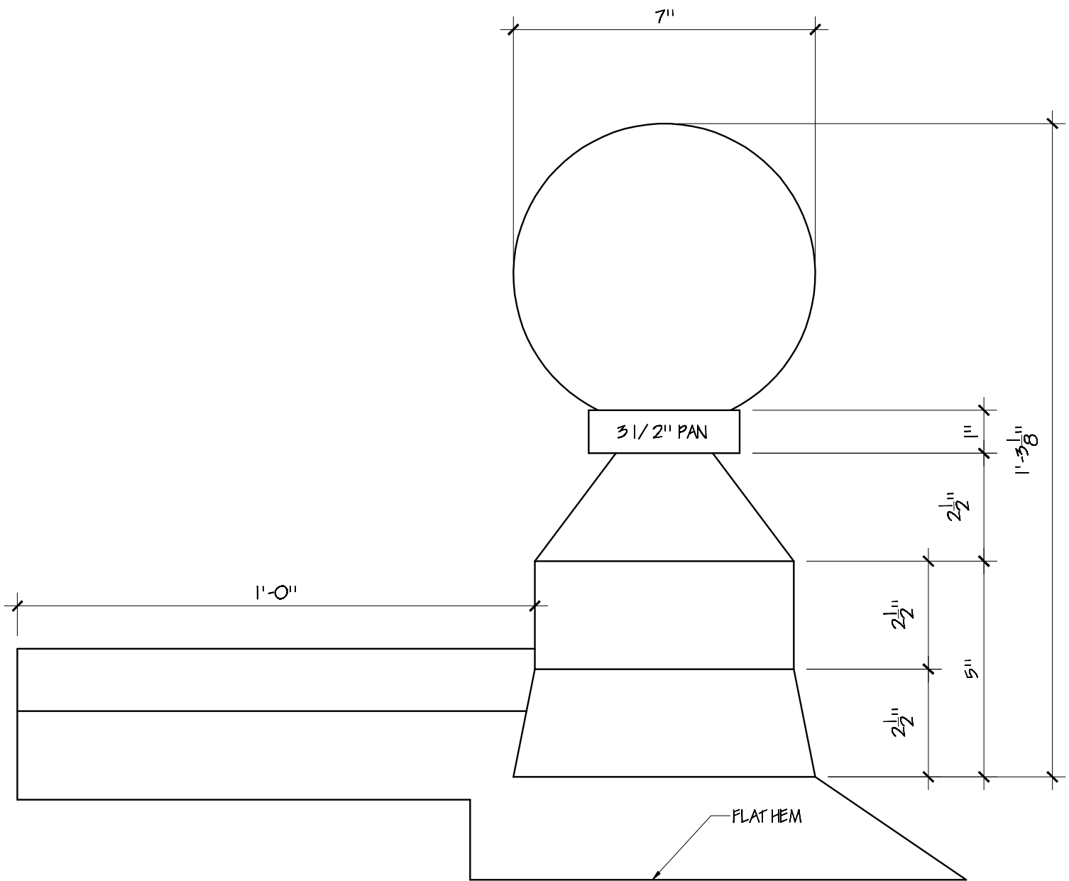
SIDE ELEVATION
