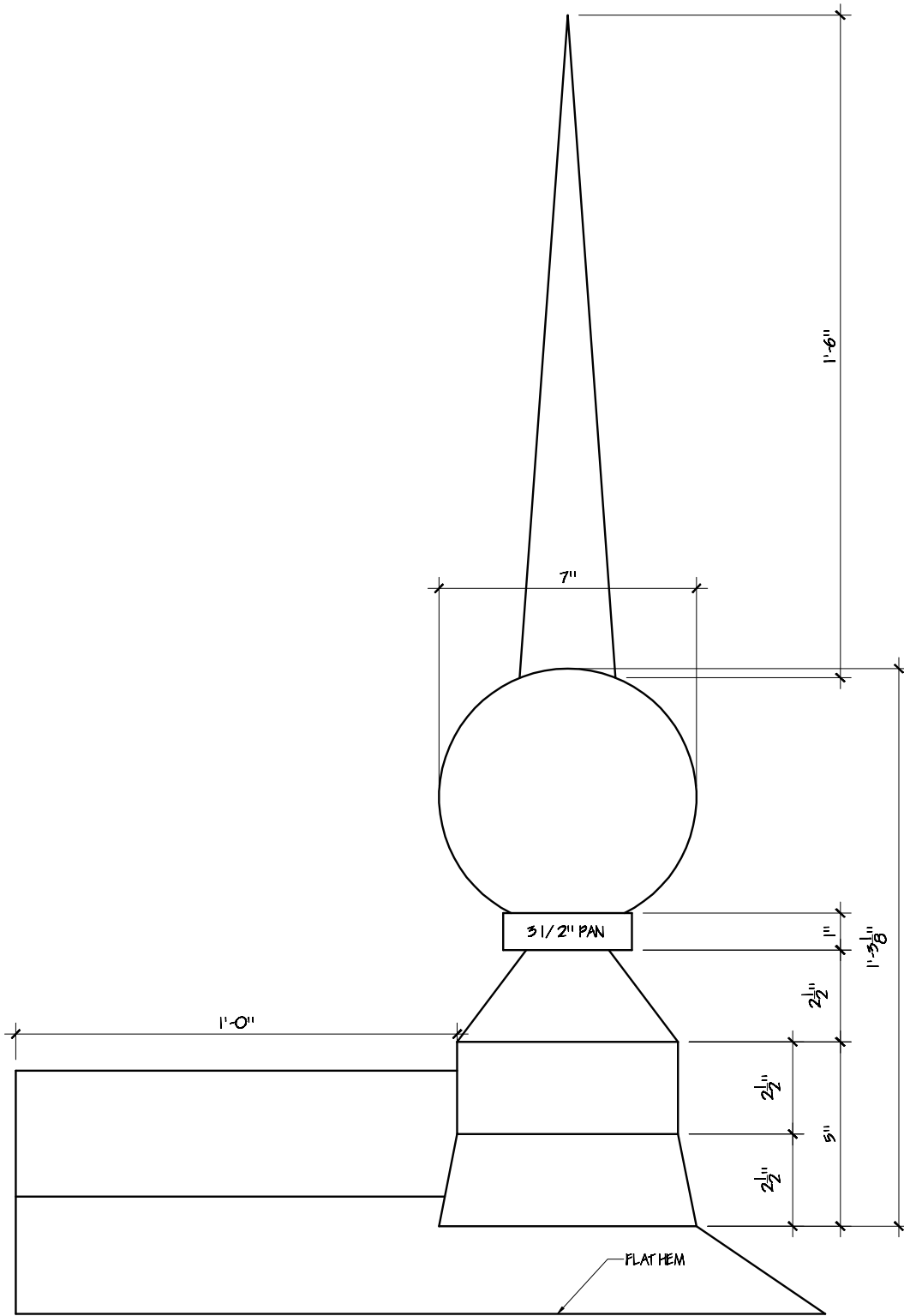
SIDE ELEVATION
