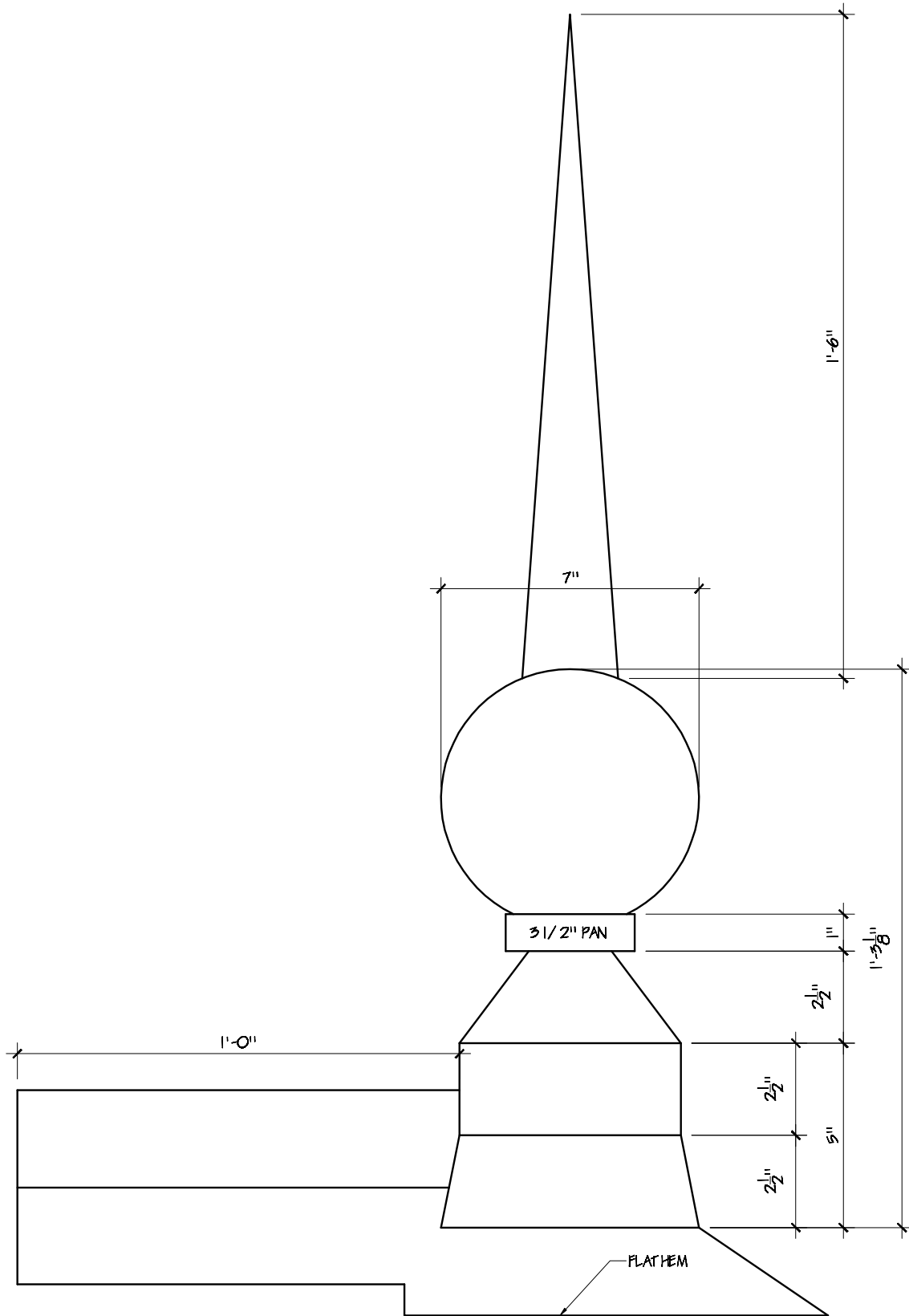
SIDE ELEVATION
