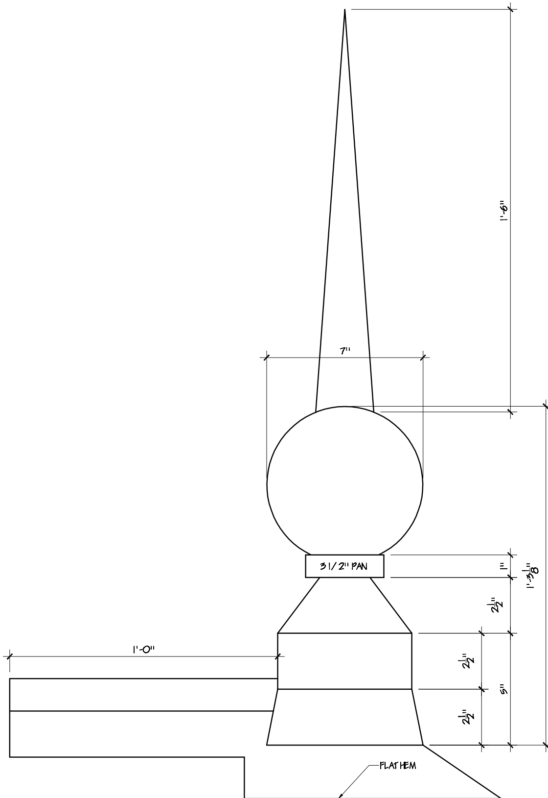
SIDE ELEVATION
