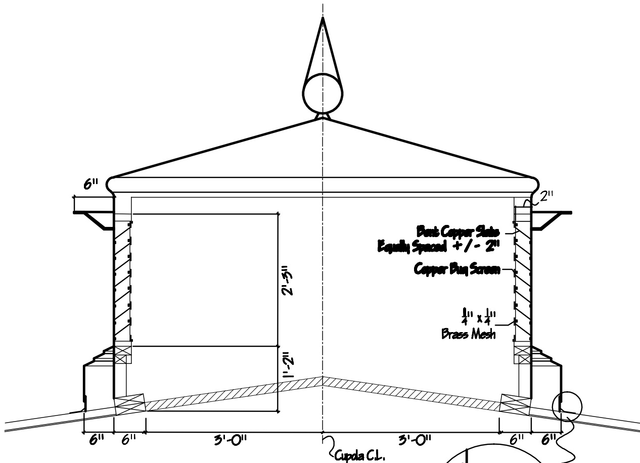
Section View
