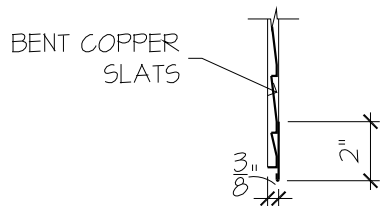
NON-VENTED SECTION
