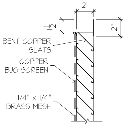
VENTED SECTION
