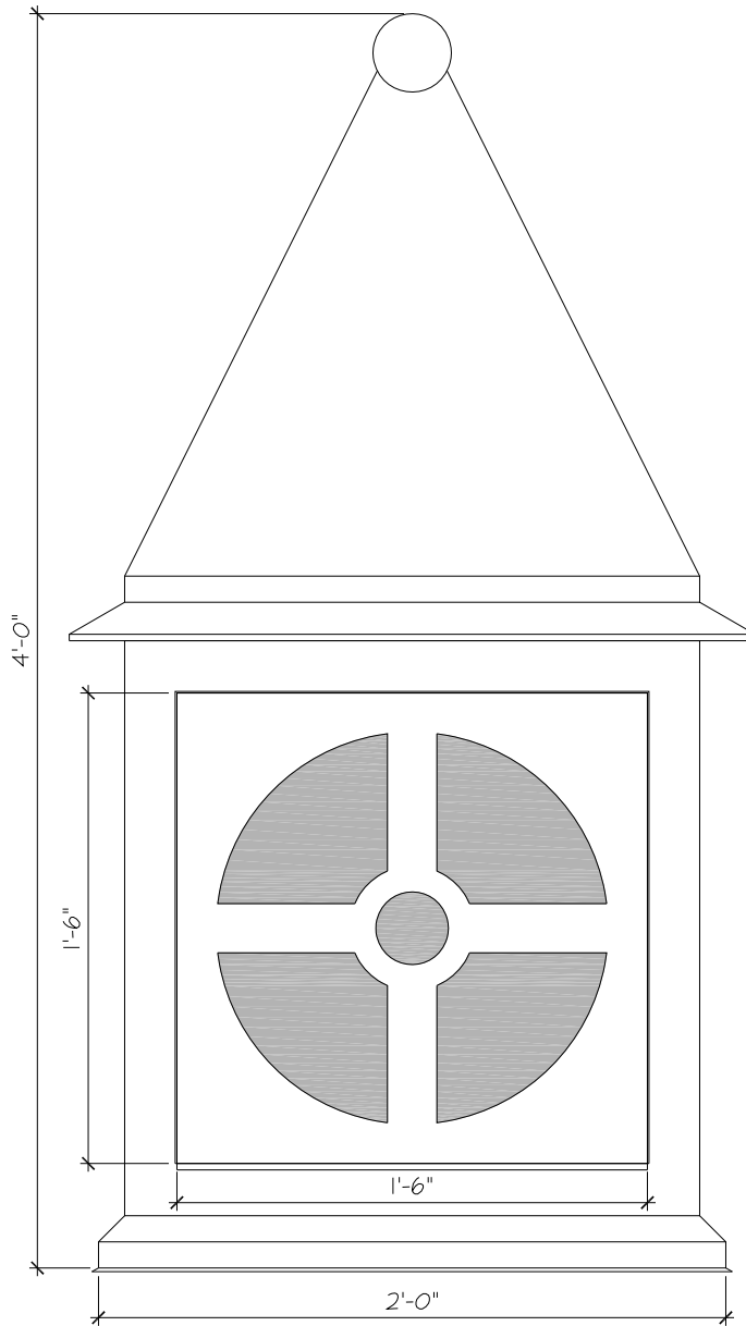
HAMPTON COVE WITH INSET - B
