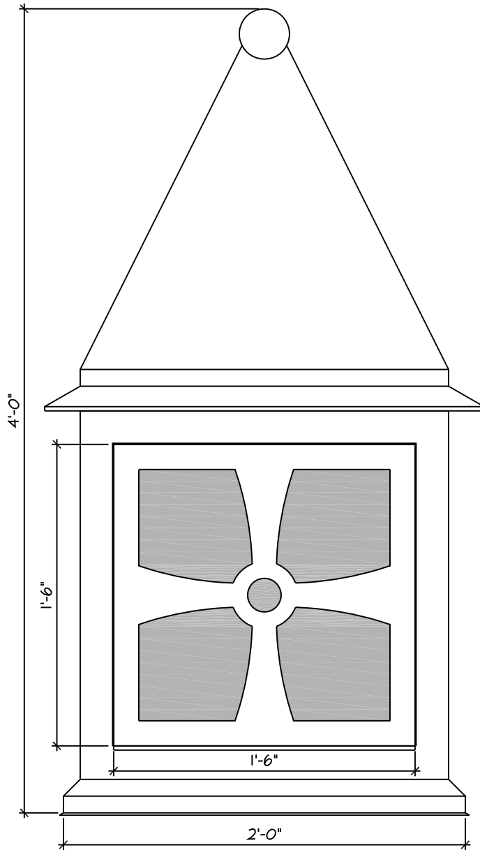
HAMPTON COVE WITH INSET - C
